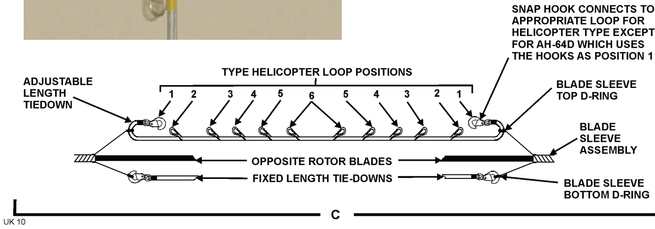
Figure 2. Blade Sleeve Assembly Rigging and Installation
